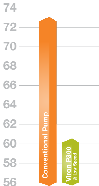
Noise Level dBA at 1 Metre Viron P300 v Conventional Pool Pump
